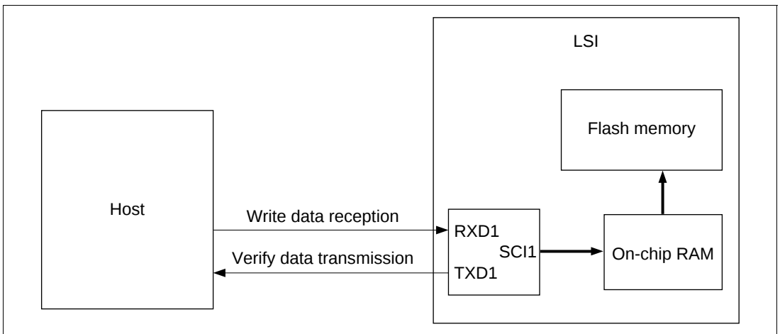
Figure 15-6 System Configuration in Boot Mode
