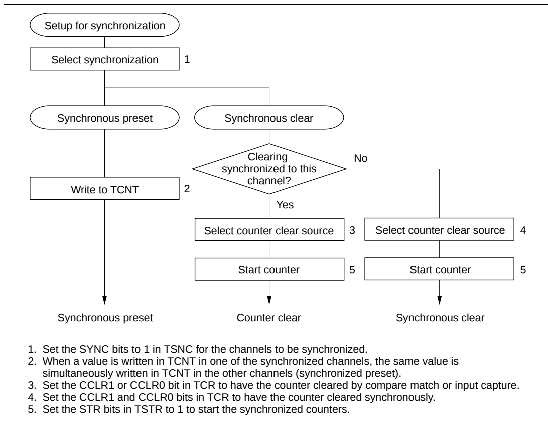
Figure 8-26 Setup Procedure for Synchronization (Example)
