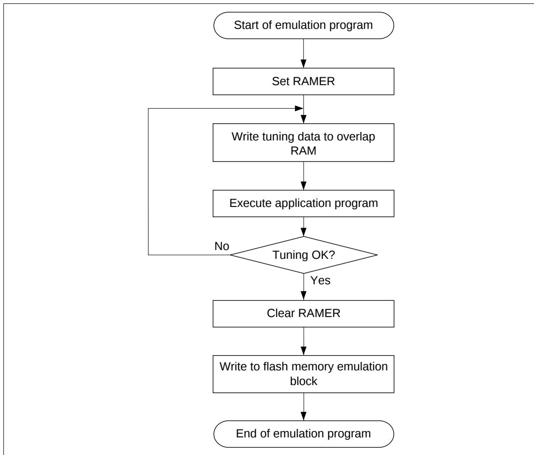
Figure 15-14 Flowchart for Flash Memory Emulation in RAM
