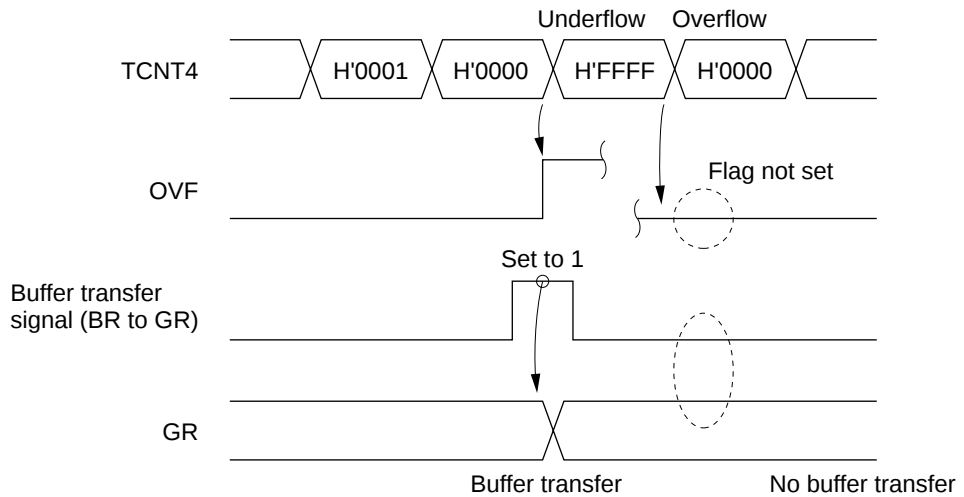
Figure 8-38 Undershoot Timing
