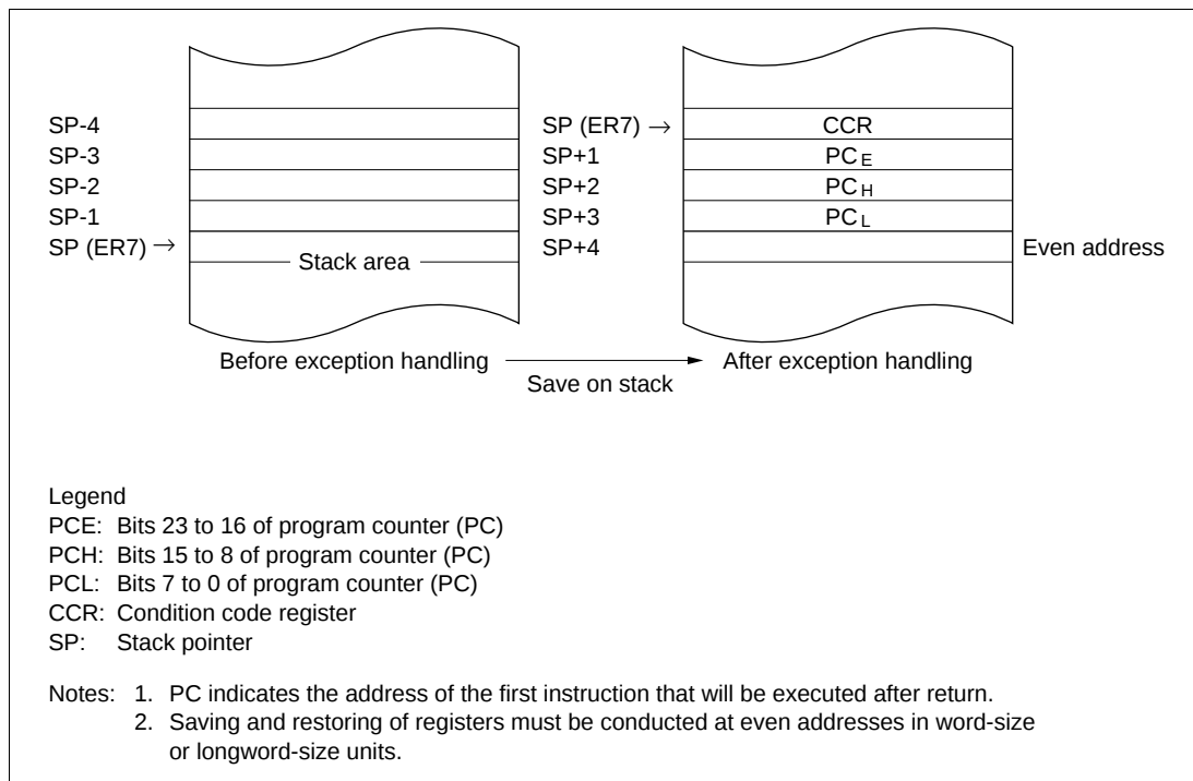
Figure 4-4 Stack after Completion of Exception Handling (Advanced Mode)
