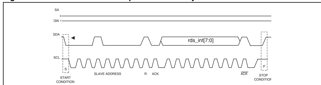
Figure 17. I 2 C read access example 2: read of 1 byte
