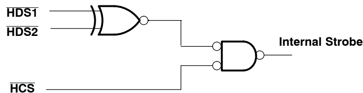
Figure 4. Select Input Logic
