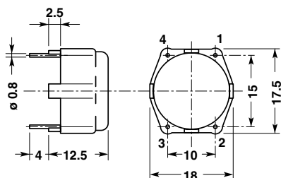
42H17 Horizontal mounting
