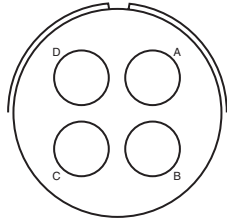
Insert Arrangement 32-17 Service Rating D Number of Contacts 4 Contact Size 4
