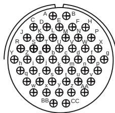
Insert Arrangement 32-48 Service Rating Inst. Number of Contacts 48 Contact Size 16
