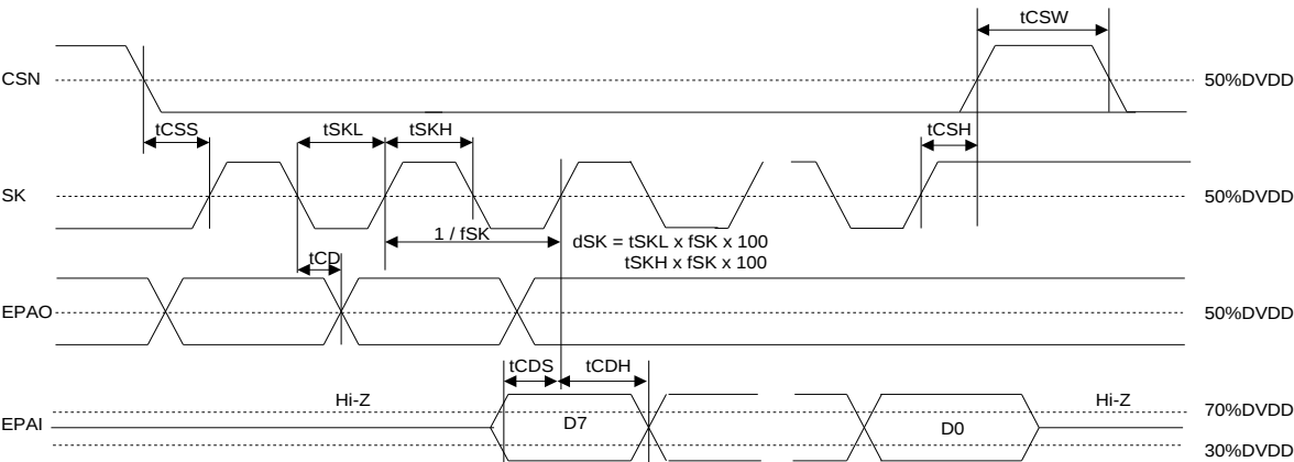
Figure 9. SPI (EEP-ROM) Control Interface Timing
