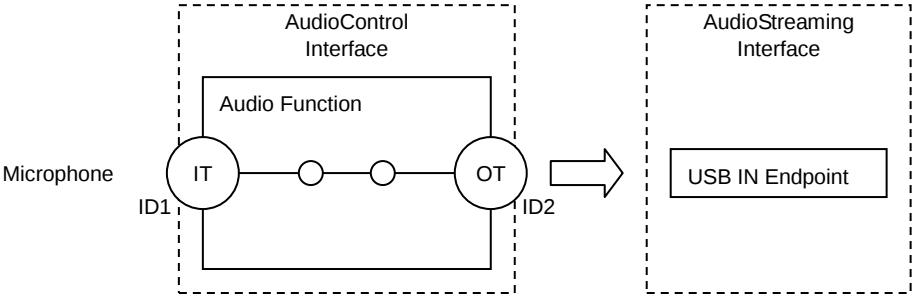
Figure 16. AK5374 Topology
