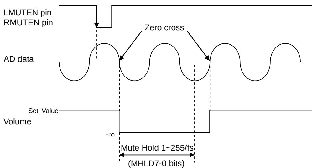
Figure 14. One Shot Mute for LMUTEN, RMUTEN pins
