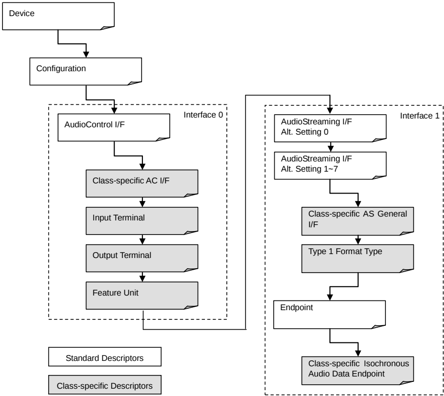
Figure 17. Descriptor Hierarchy
