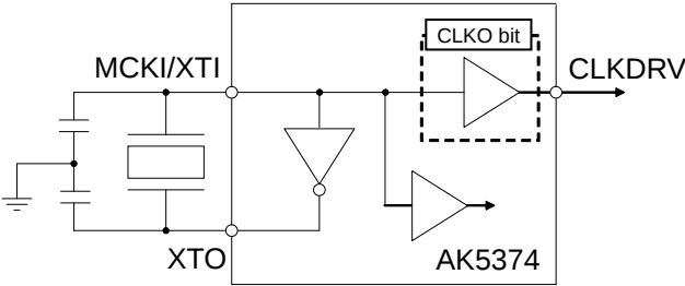
Note 17. External capacitance depends on the crystal oscillator (Max. 30pF) Figure 10. X'tal Mode
