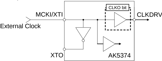
Note 18. Input clock must not exceed DVDD. Figure 11. External clock mode
