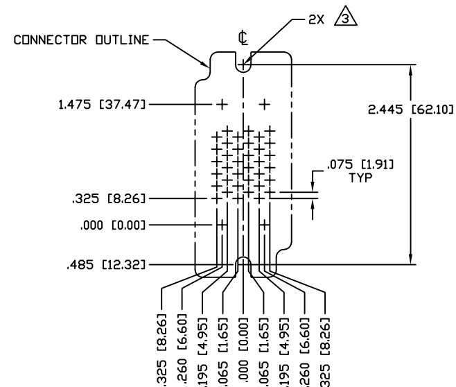
RECOMMENDED CONTACT LAYOUT AS VIEWED FROM CONNECTOR MOUNTING SIDE (FRONT VIEW)
