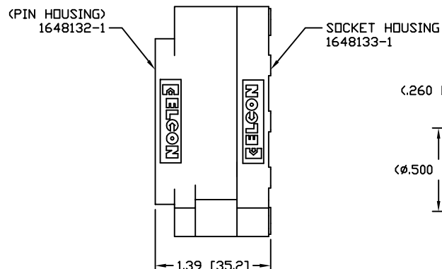
MATED CONDITION
