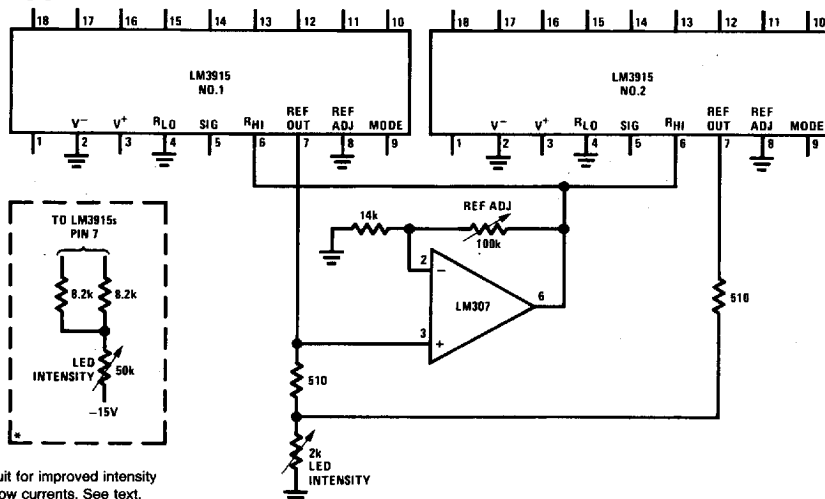
FIGURE 10. Wide-Range Adjustment of Reference Voltage and LED Intensity for Multiple LM3915s
