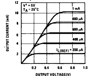
Output Characteristics
