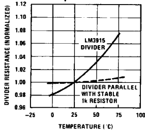
Total Divider Resistance vs Temperature
