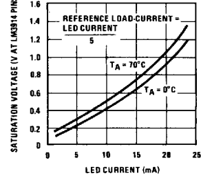
LED Driver Current Regulation
