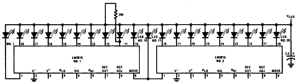
Cascading LM3915s in Dot Mode
