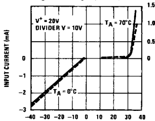
Input Current Beyond Signal Range (Pin 5)
