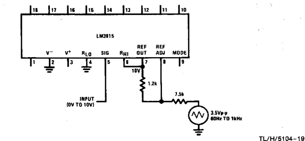
FIGURE 11. 0V to 10V Log Display with Smooth Transitions
