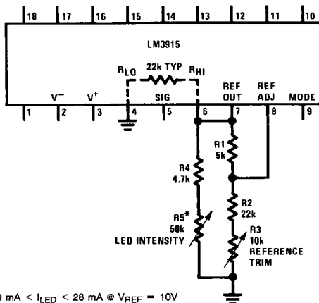
FIGURE 8. Varying LED Intensity
