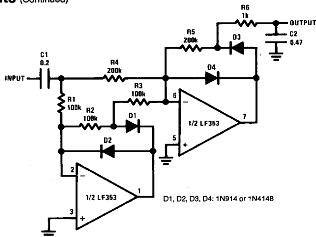
FIGURE 4. Precision Full-Wave Peak Detector
