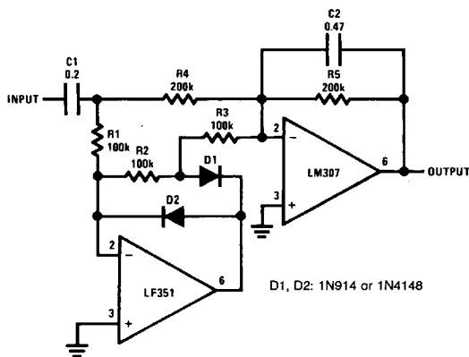
FIGURE 3. Precision Full-Wave Average Detector
