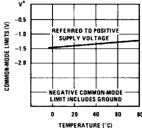
Common-Mode Limits
