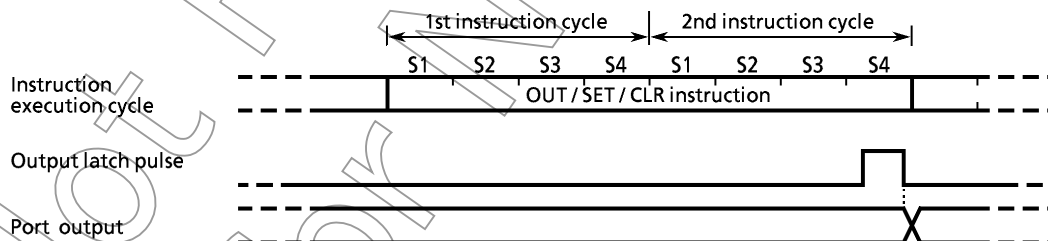
Figure 3-2. Output Timing
