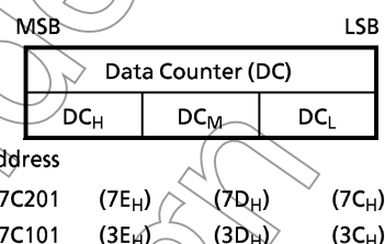
Figure 2-7. Data Counter
