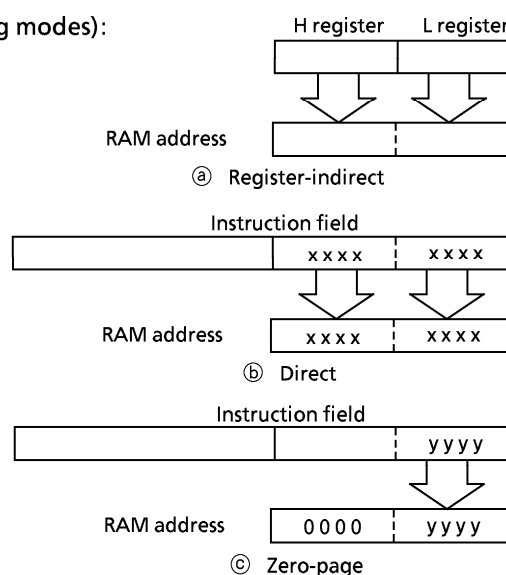
Figure 2-5. Addressing mode
