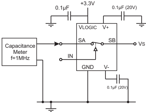
Figure 9 - On Capacitance
