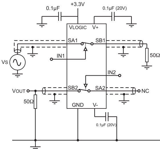
Figure 7 - Channel-to-Channel Crosstalk
