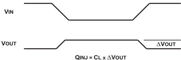
Figure 5. Charge Injection
