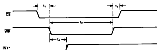
Figure 1. AD7579/AD7580 Start Cycle Timing
