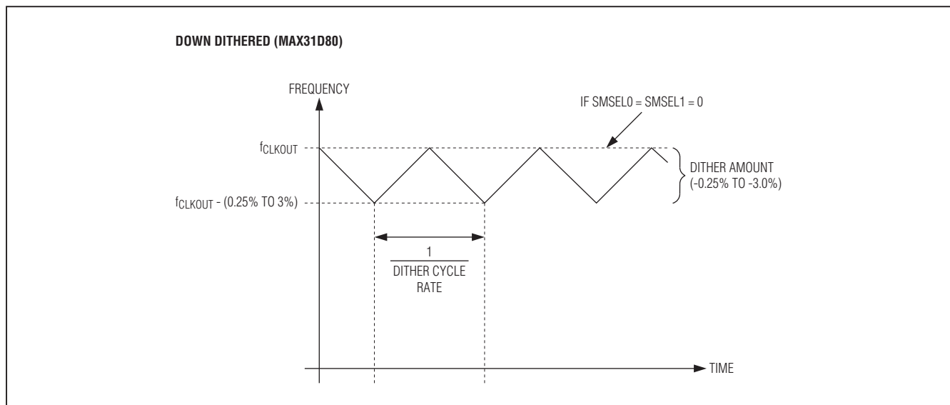
Figure 1. Spread-Spectrum Frequency Modulation (Down Dithered)
