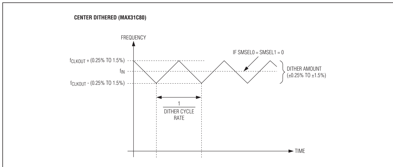
Figure 2. Spread-Spectrum Frequency Modulation (Center Dithered)
