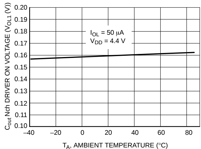
Figure 14. Cout Nch Driver On Voltage vs. Temperature
