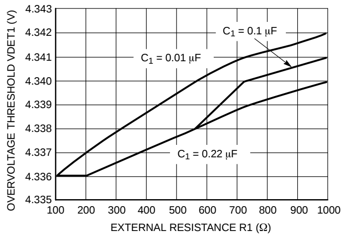
Figure 21. Overvoltage Threshold vs. External Resistance R1
