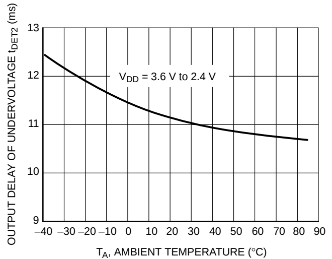
Figure 8. Output Delay of Undervoltage vs. Temperature
