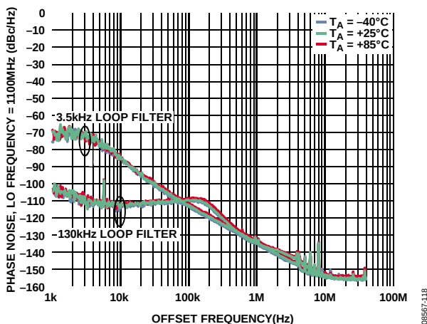
Figure 18. Phase Noise vs. Offset Frequency and Temperature, f_{LO} = 1100 MHz
