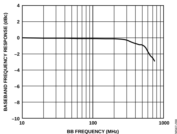
Figure 39. Baseband Bandwidth
