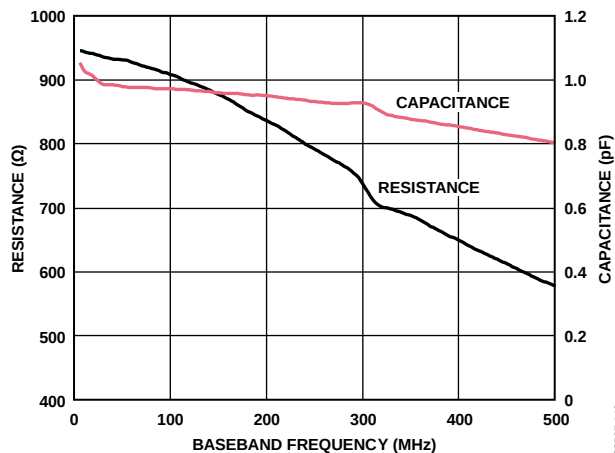
Figure 40. Differential Baseband Input R and C (Shunt R, Shunt C)
