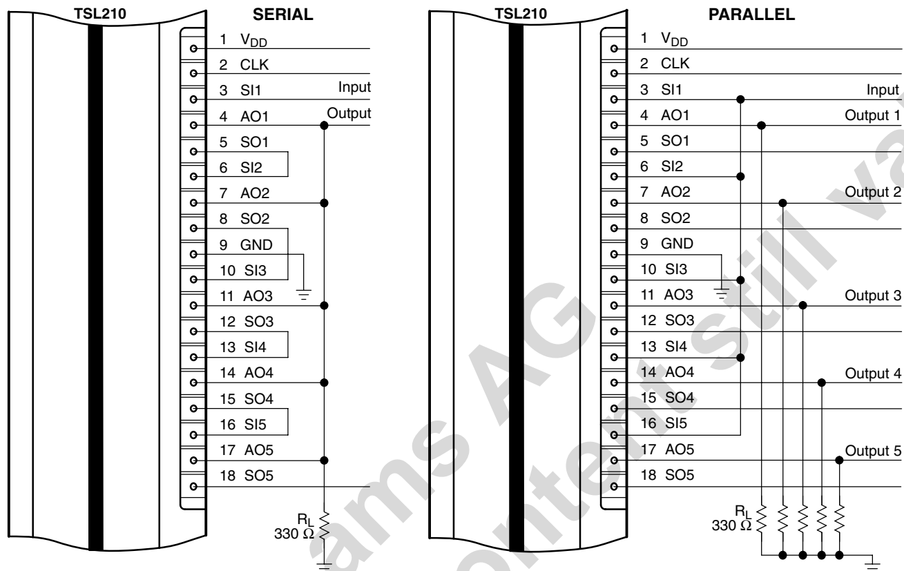
Figure 4. Connection Diagrams
