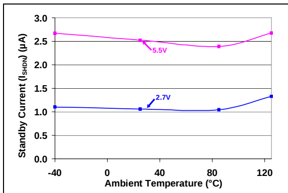
FIGURE 2-2: Device Current ( I_{SHDN} ) and V_{DD} ( \text{HVC/A0} = V_{DD} ) vs. Ambient Temperature.
