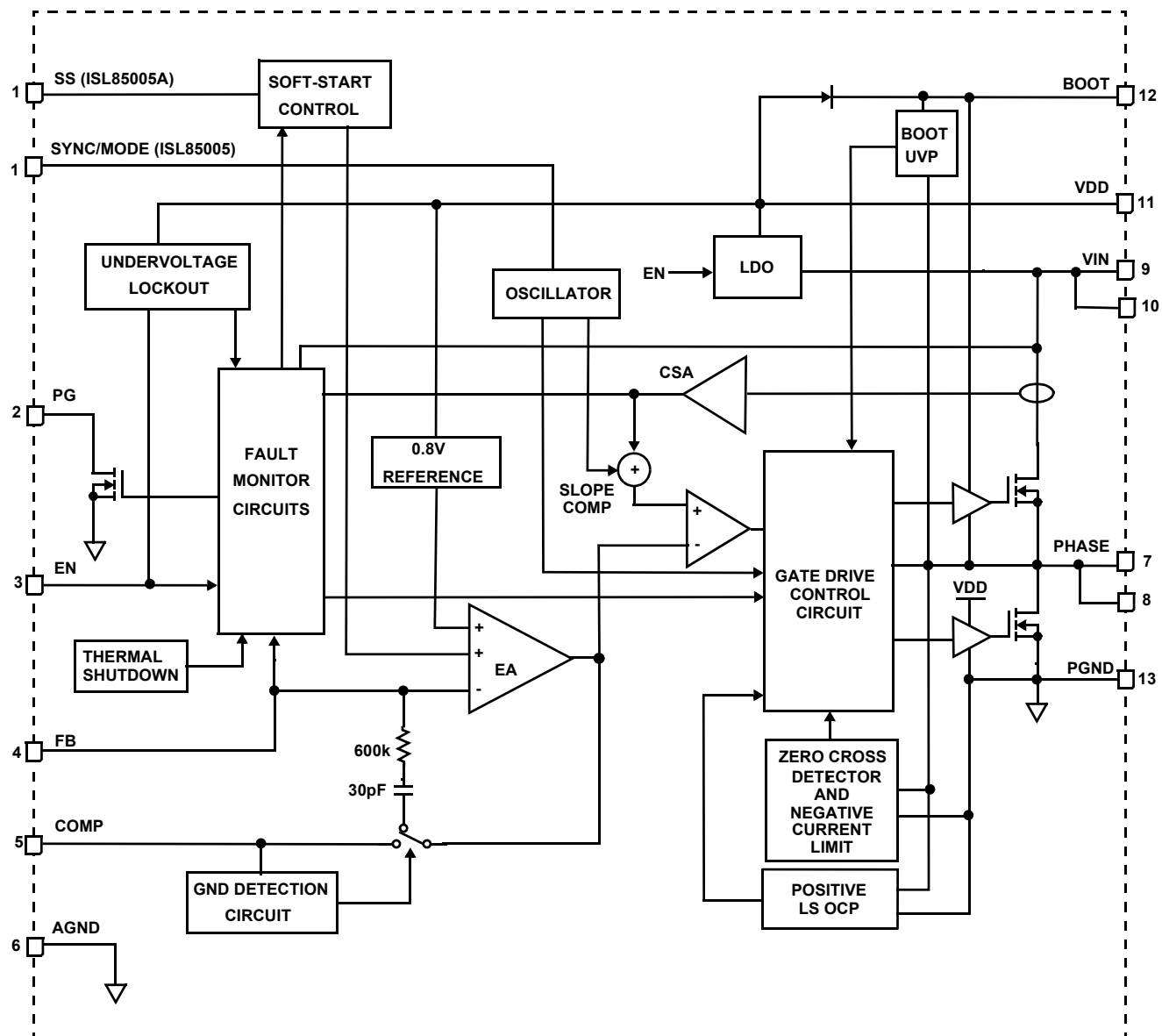
FIGURE 3. BLOCK DIAGRAM
