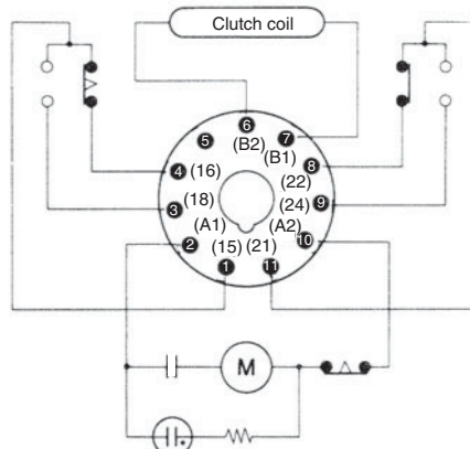
H2C(-F)R/H2C-R-S
