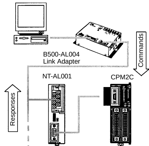
1:N Host Link Communications
