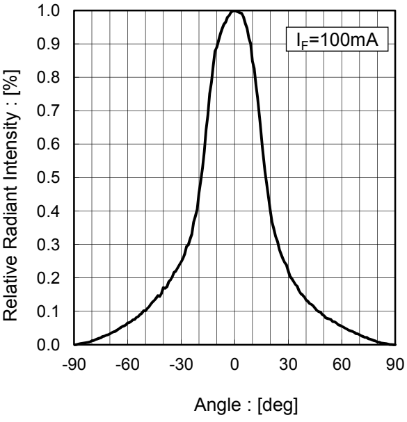
Fig.6 Radiant intensity
