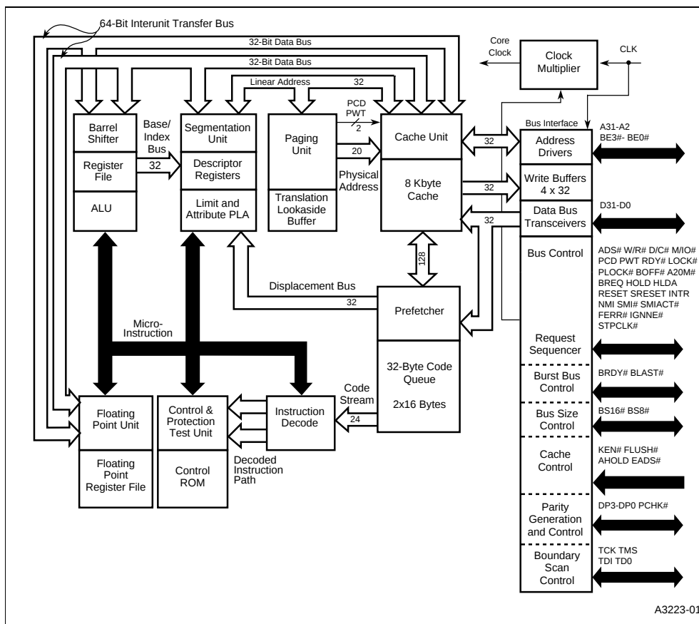
Figure 1. Embedded IntelDX2™ Processor Block Diagram
