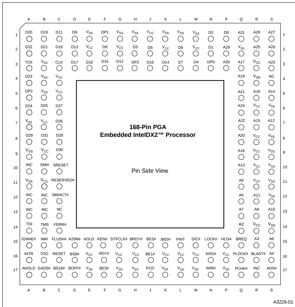
Figure 3. Package Diagram for 168-Pin PGA Embedded Intel® X2™ Processor
