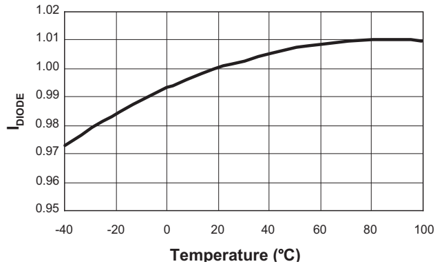
Normalized I_{DIODE} vs. Temperature
