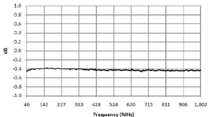
MABA-011030 Insertion Loss 2 (pin4-1)
