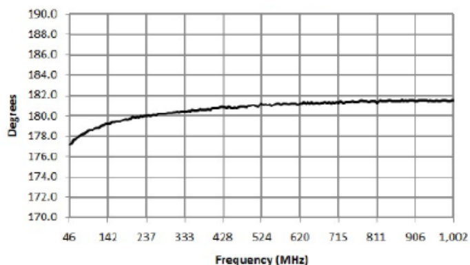
MABA-011030 Phase Balance
