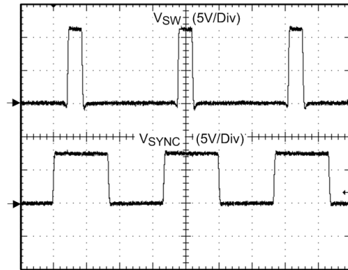
Figure 16. Frequency Synchronization
