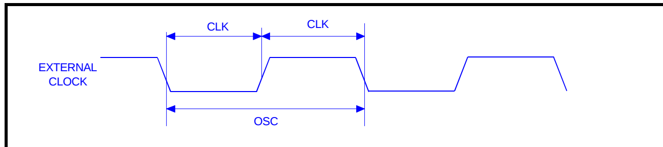
FIGURE 11. CLOCK TIMING
