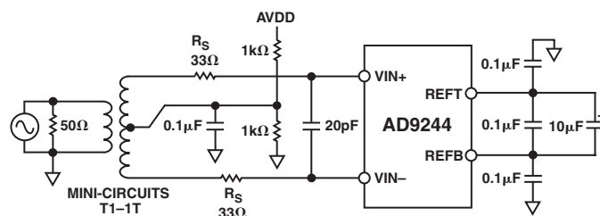
Figure 7. Transformer-Coupled Input
