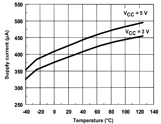
Figure 2. Supply current/amplifier vs. temperature
