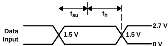
VOLTAGE WAVEFORMS SETUP AND HOLD TIMES
