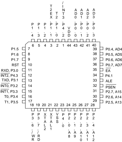
44-Pin PLCC
