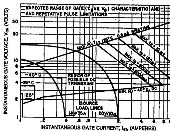
GATE CHARACTERISTICS
