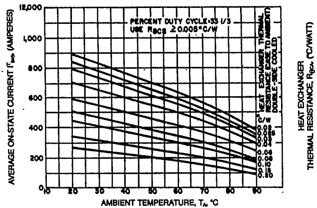
I_{T(av)} vs. T_A (VARIOUS HEAT EXCHANGERS) (RECTANGULAR WAVEFORM)
