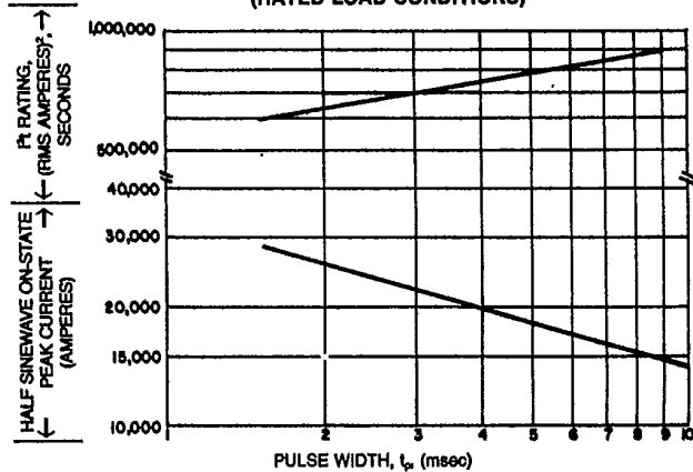
SUB-CYCLE SURGE AND I_{T(av)} RATINGS (RATED LOAD CONDITIONS)
