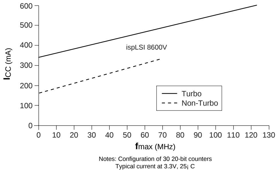
Figure 10. Typical Device Power Consumption vs fmax
