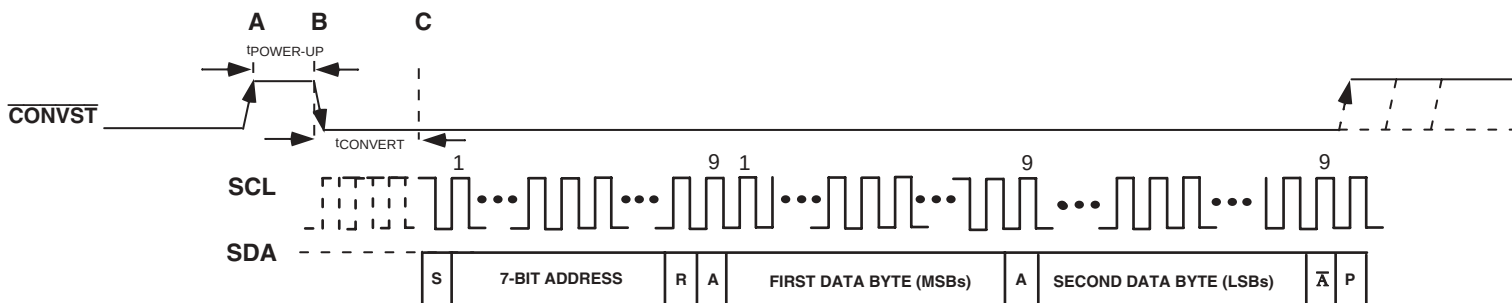
Figure 16. Mode 1 Operation
