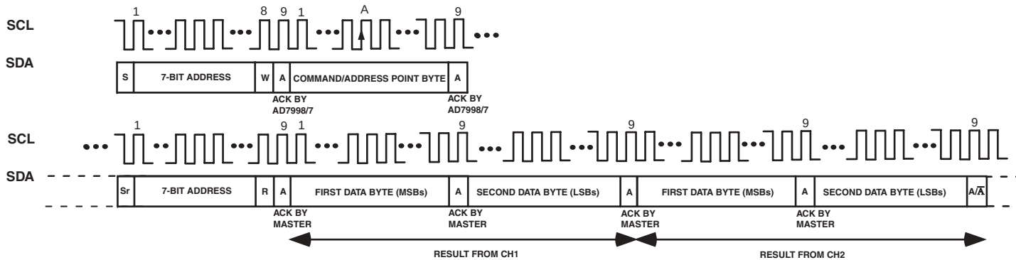
Figure 17. Mode 2 Operation
