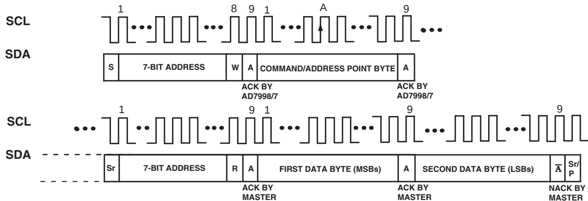
Figure 17. Mode 2 Operation
