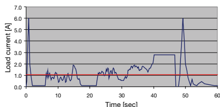
Figure 4: Garden shredder
