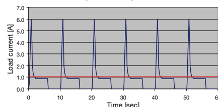
Figure 2: Feeder
