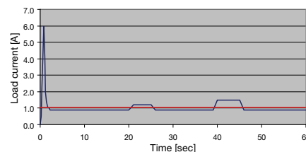
Figure 3: Ventilator
