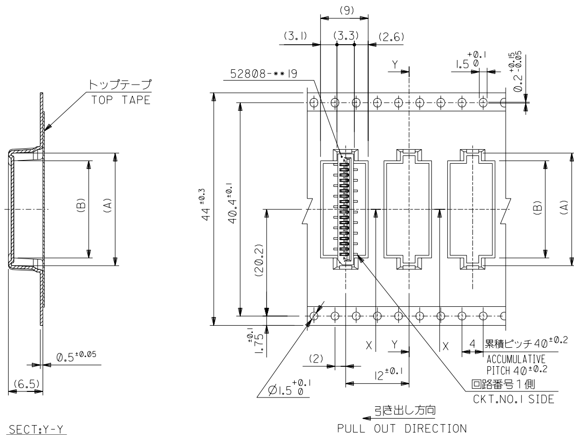
SECT:Y-Y
