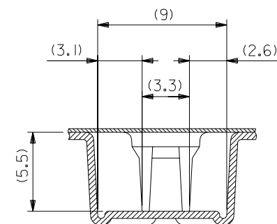
SECT:X-X (SCALE:4-1)
