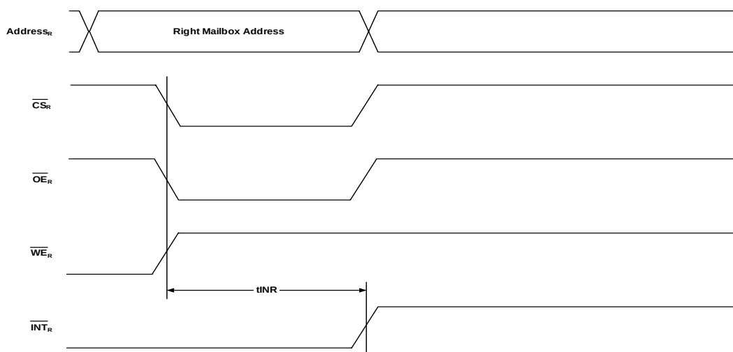
Right Port Reads Right Mailbox Clearing \overline{INT}_R
