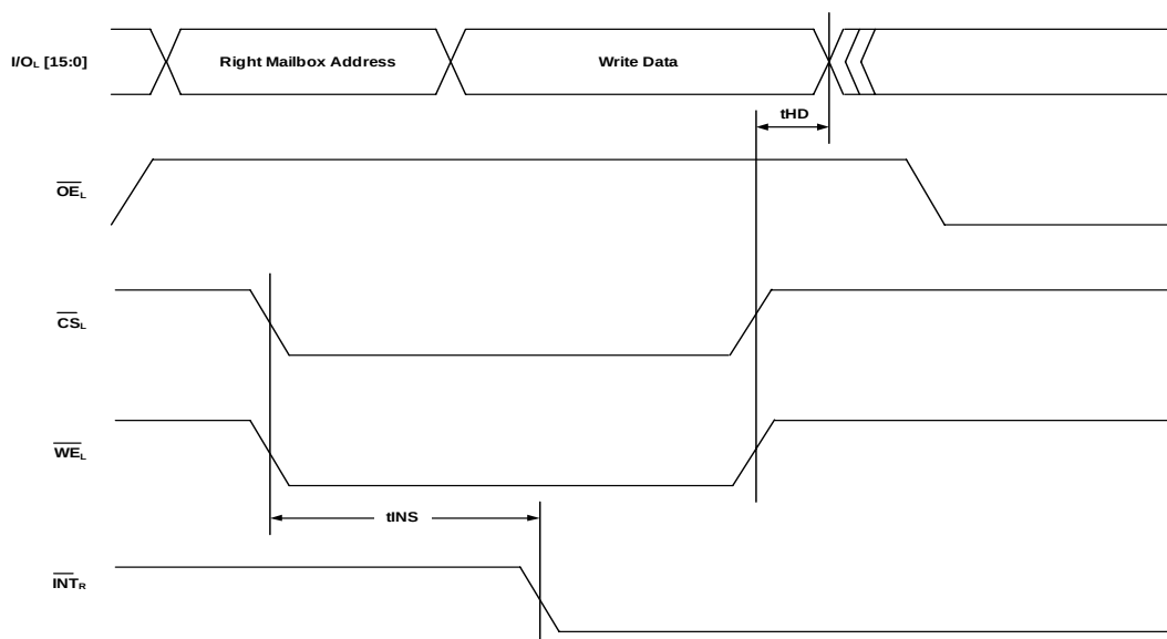
Left Port Writes to Right Mailbox Setting \overline{INT}_R
