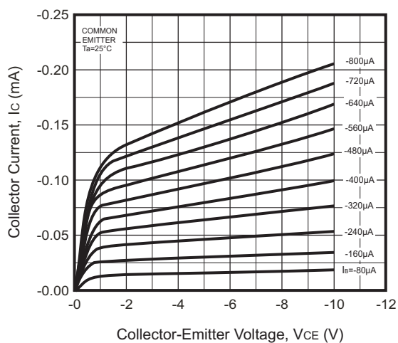
Fig.1 - Static Characteristic
