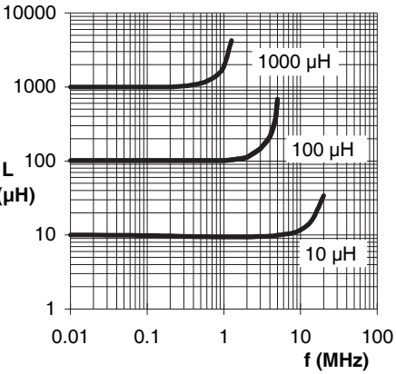
Typical L vs Frequency(f)
