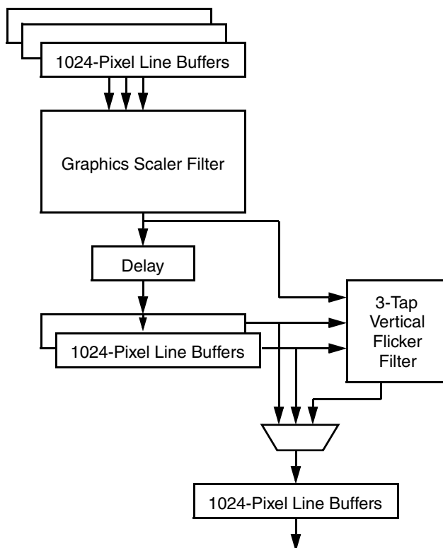
Figure 6-21. Flicker Filter and Line Buffer Path
