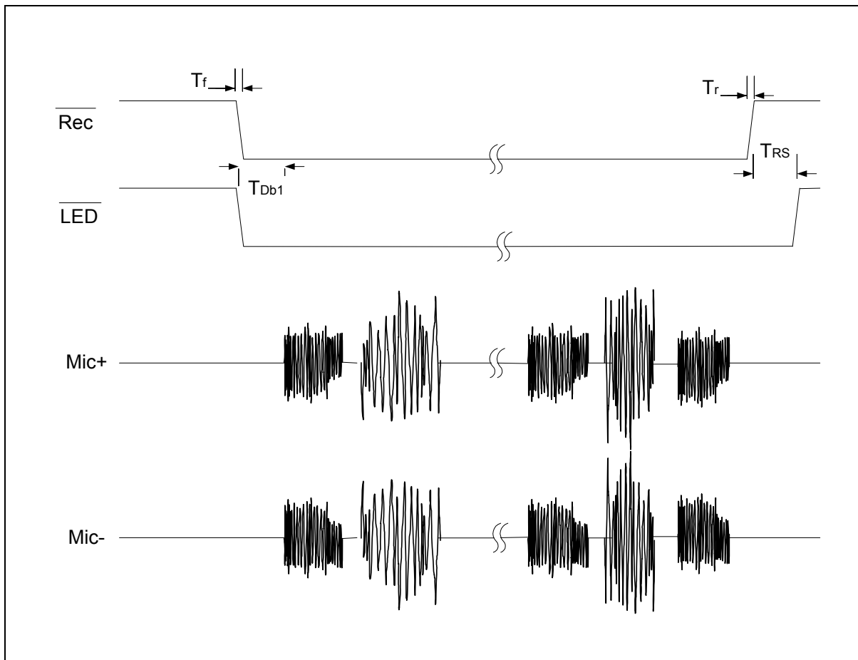
FIGURE 1: RECORD OPERATION
