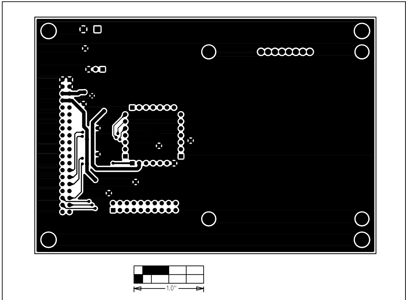
Figure 12. MAX1234 EV Kit PC Board Layout—Solder Side
