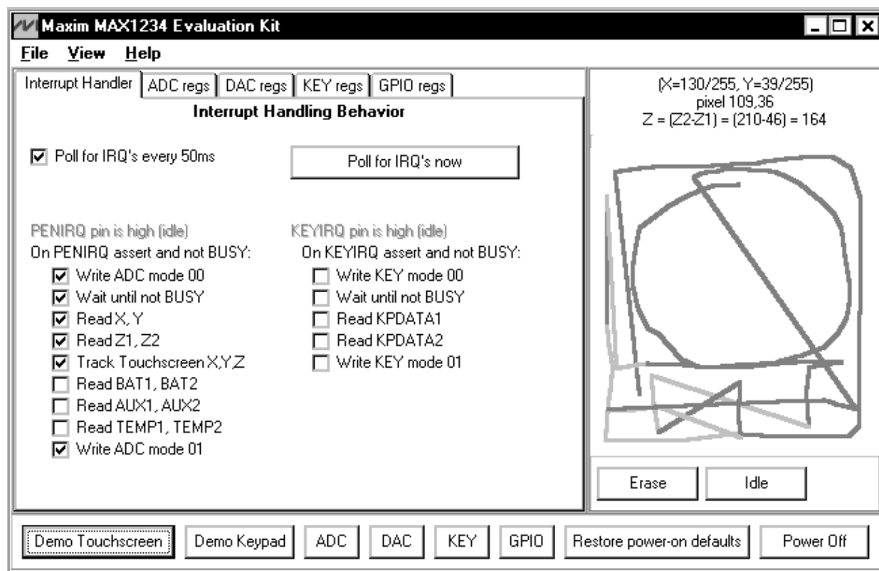
Figure 1. EV Software's Main Window
