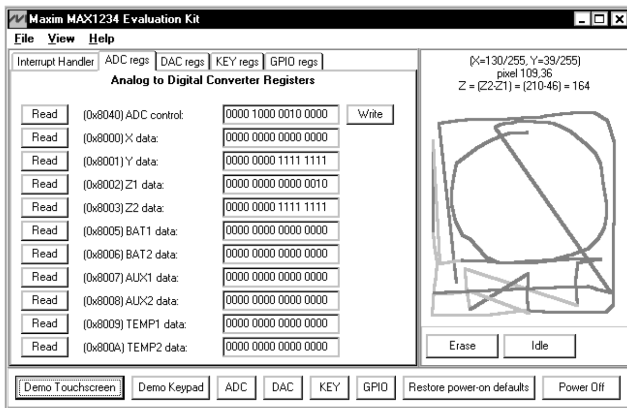
Figure 2. EV Software's Main Window
