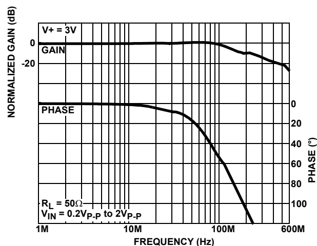
FIGURE 19. FREQUENCY RESPONSE
