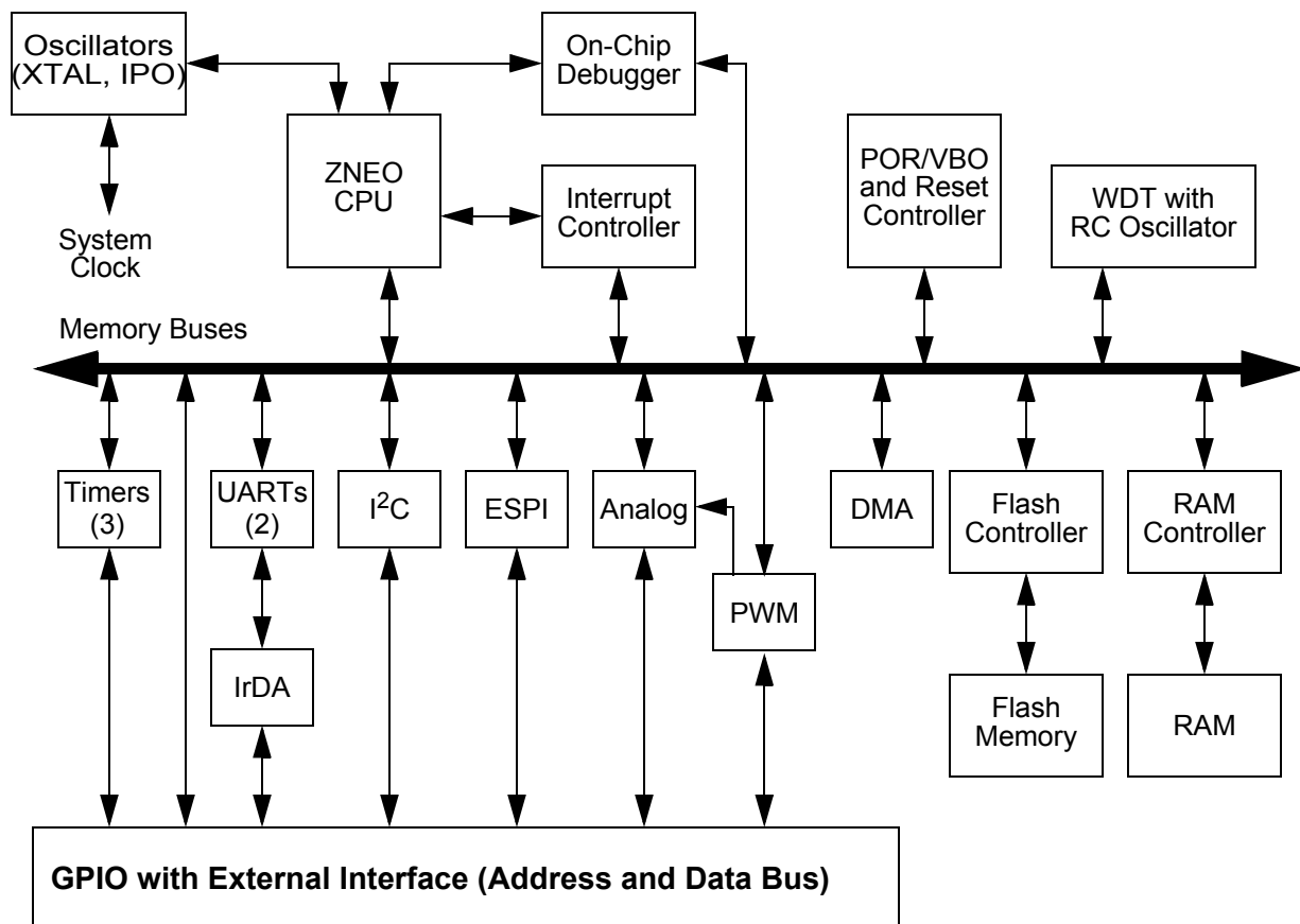
Figure 1. ZNEO Z16F Series Block Diagram
