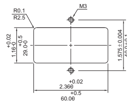
SUGGESTED MOUNTING CUTOUT
