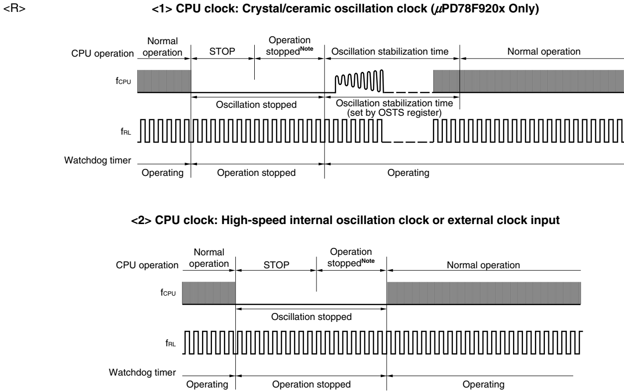
Figure 8-7. Operation in STOP Mode (WDT Operation Clock: Low-Speed Internal Oscillation Clock)
