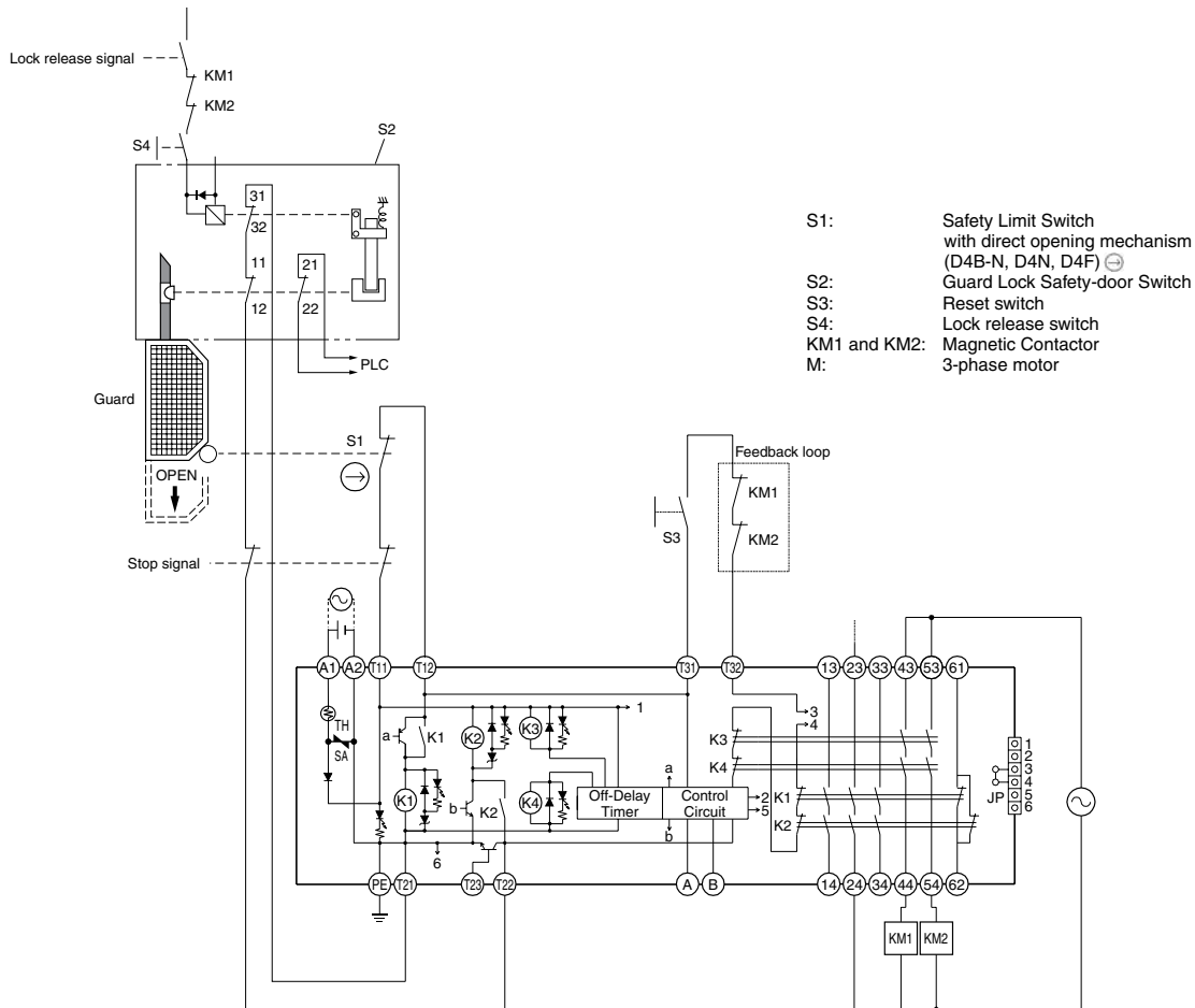
G9SA-321-T□ (24 VAC/VDC) + D4BL-□D□A-□, - □D□B-□ (Mechanical Lock Type) Circuit Diagram (Manual Reset)a
