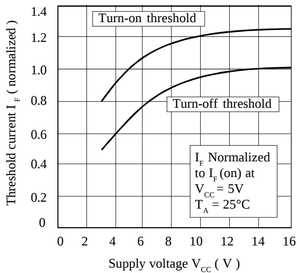
Threshold Current vs. Supply Voltage
