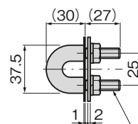
2- M8×40六角穴付き止ねじ Hex socket set screw
