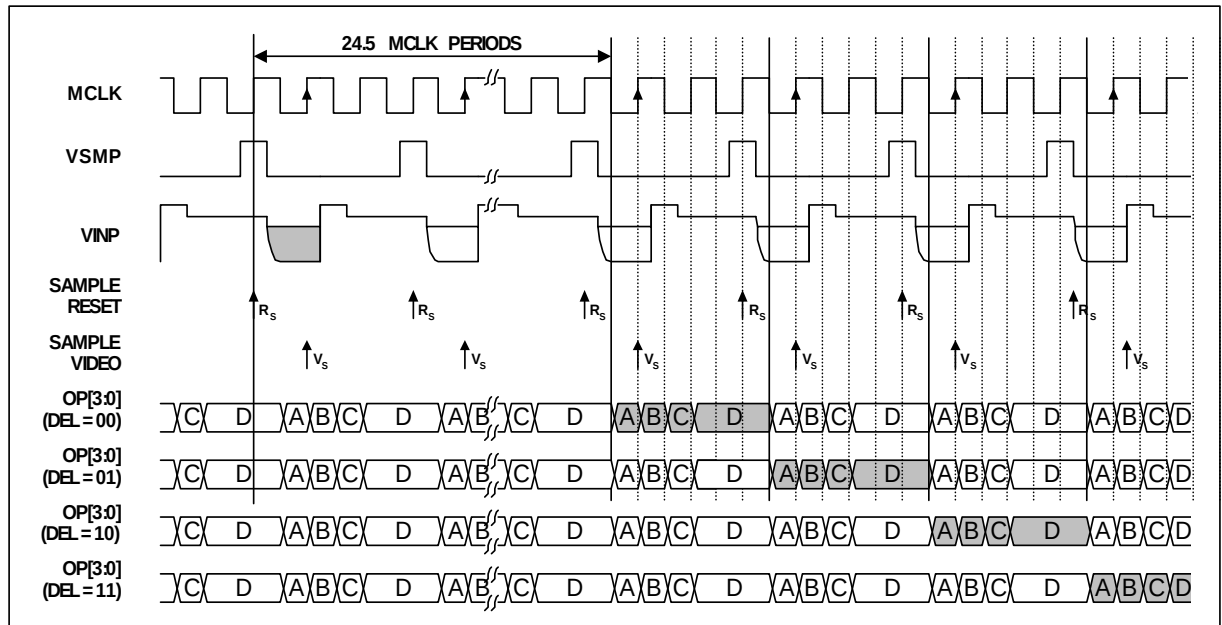
Figure 15 Mode 2 Operation
