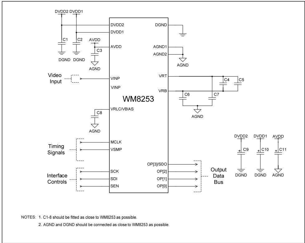
Figure 18 External Components Diagram
