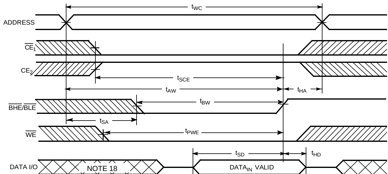
Write Cycle No. 4 ( \overline{\text{BHE/BLE}} Controlled, \overline{\text{OE}} LOW) [17]
