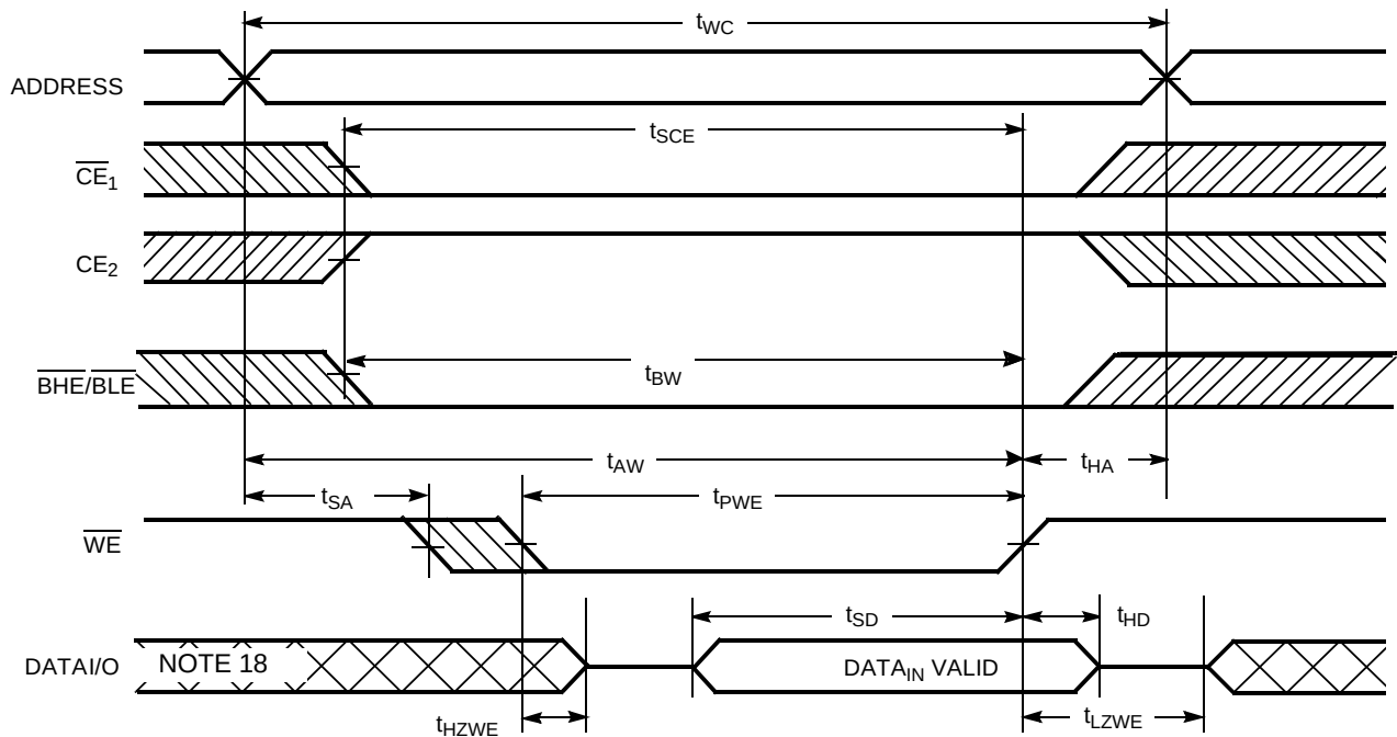
Write Cycle No. 3 ( \overline{\text{WE}} Controlled, \overline{\text{OE}} LOW) [17]
