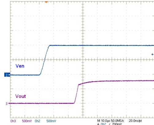
Figure 15. Enable transient
